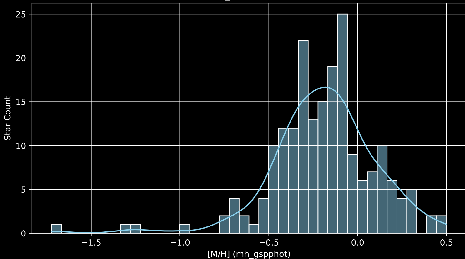
APOGEE DR17 Field: [172+27_MGA [M/H] (mh_gspphot) (n= 196)
