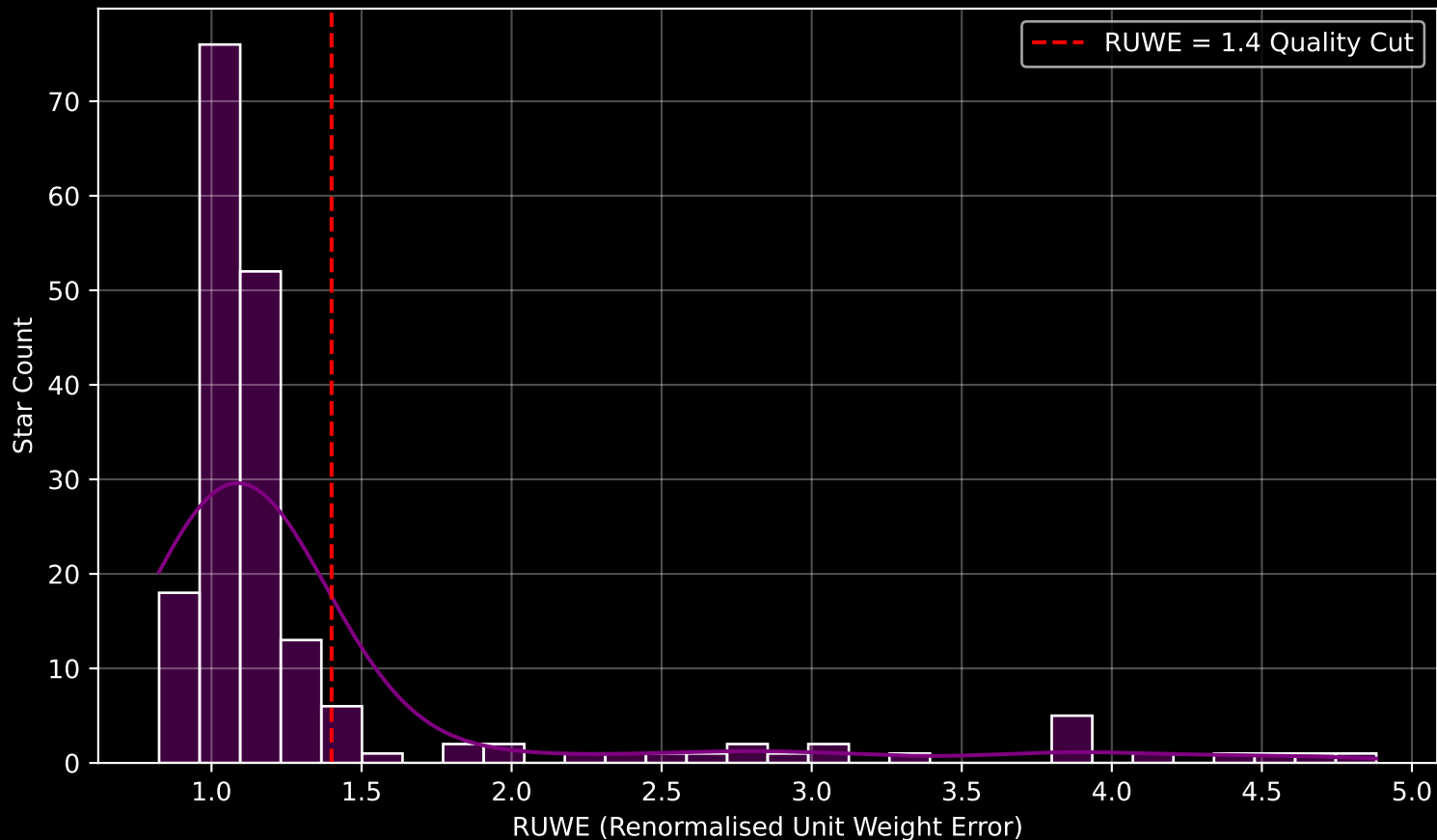
GAPOGEE DR17 Field [172+27_MGA] RUWE Distribution (n= 190)
