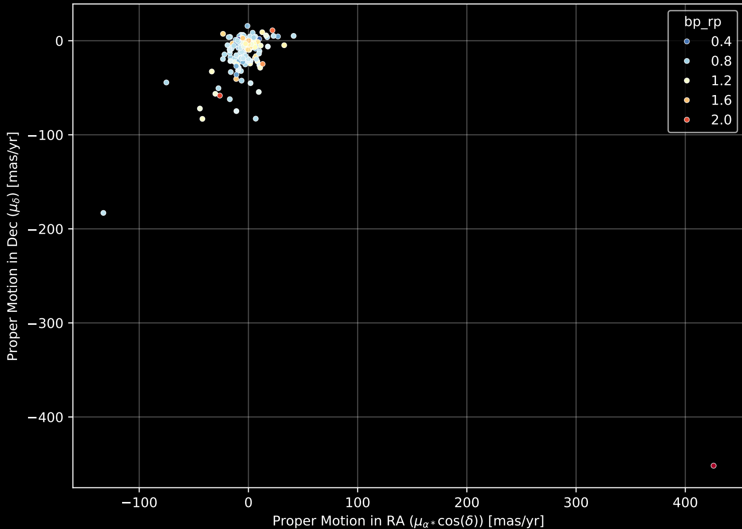
APOGEE DR17 Field: [172+27_MGA] Proper Motion Diagram (n= 197)
