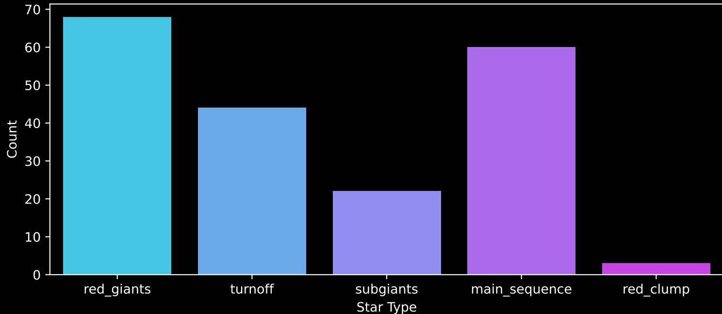
APOGEE DR17 Field: [172+27_MGA] Count plot of Star Type
