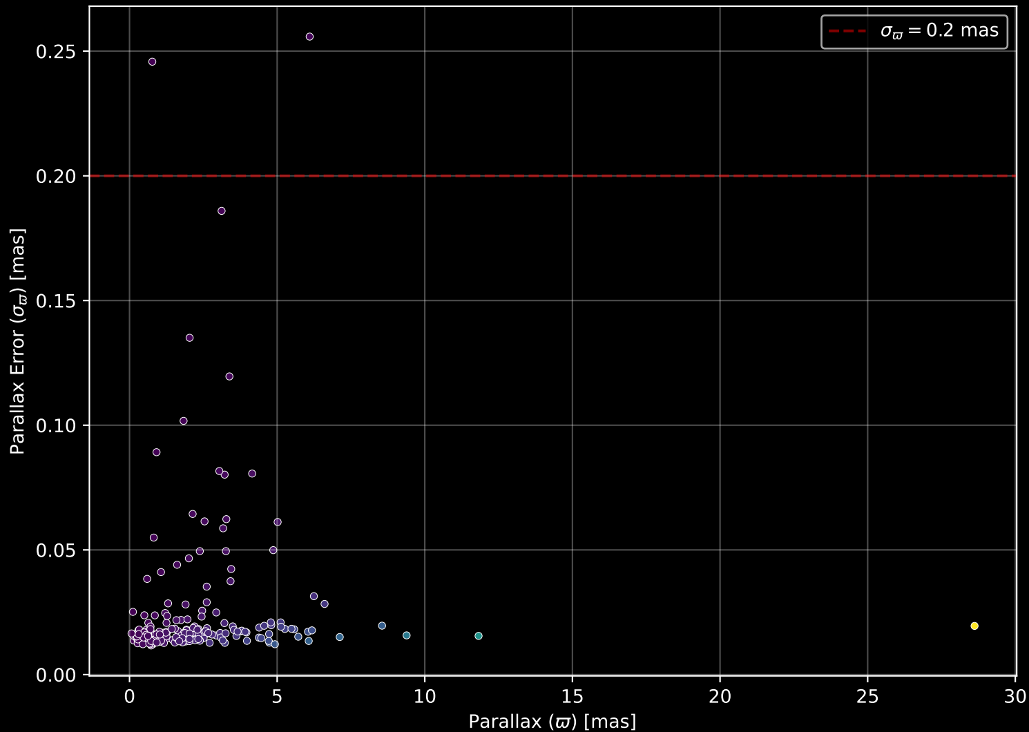
APOGEE DR17 Field: [172+27_MGA] Parallax Quality (n= 197)
