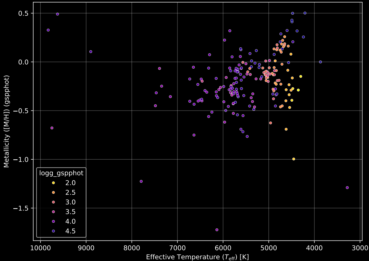
APOGEE DR17 Field: [172+27_MGA] Stellar Population Parameters (n= 197)
