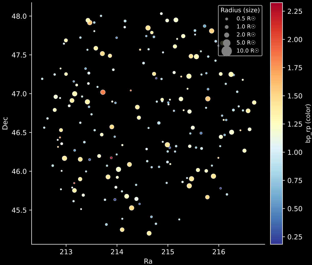
APOGEE DR17 Field: [172+27_MGA] Stars: 197
